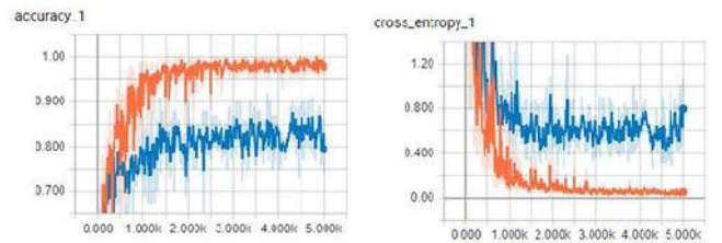
Fig. 7. The graph of the accuracy and the cross-entropy graph of MobileNet.
