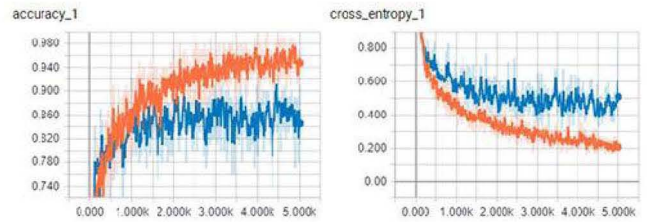
Fig. 6. The graph of the accuracy and the cross-entropy graph of Inception-V3.
