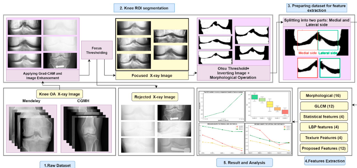
Fig. 2. Methodology workflow.
