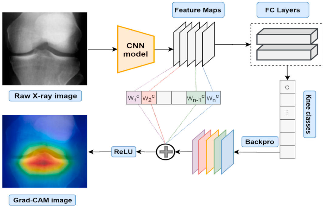
Fig. 6. Grad-CAM overview.
